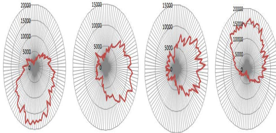
Fig. 6: Heat flux density distribution as calculated by Mathematica using results obtained from Tonatiuh at the four pipes on 15 July, 2015, in \text{W m}^{-2}
