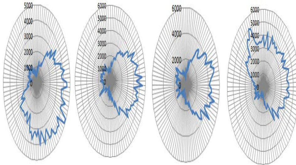
Fig. 7: Heat flux density distribution as calculated by Mathematica using results obtained from Tonatiuh at the four pipes on 30 January, 2016, in \text{W m}^{-2}
