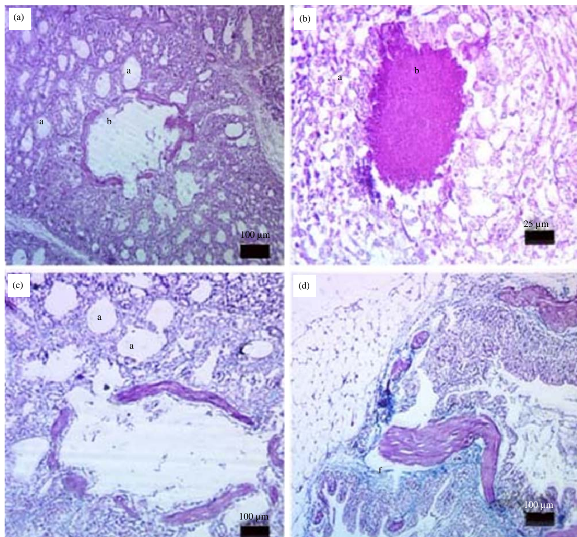
Fig. 2(a-d): Lung tissues section of infected birds and control staining with periodic acid-Schiff reaction and Masson's trichrome staining whereas, (a) Lung sections from negative lungs revealed weak PAS reaction, (b) Lung sections from the infected group revealed strong PAS reaction, (c) Lung sections showed few collagen fibers around the bronchioles and alveoli (d) Lung sections showed excessive collagen fibers with decreased thickness and staining of elastic fibers
