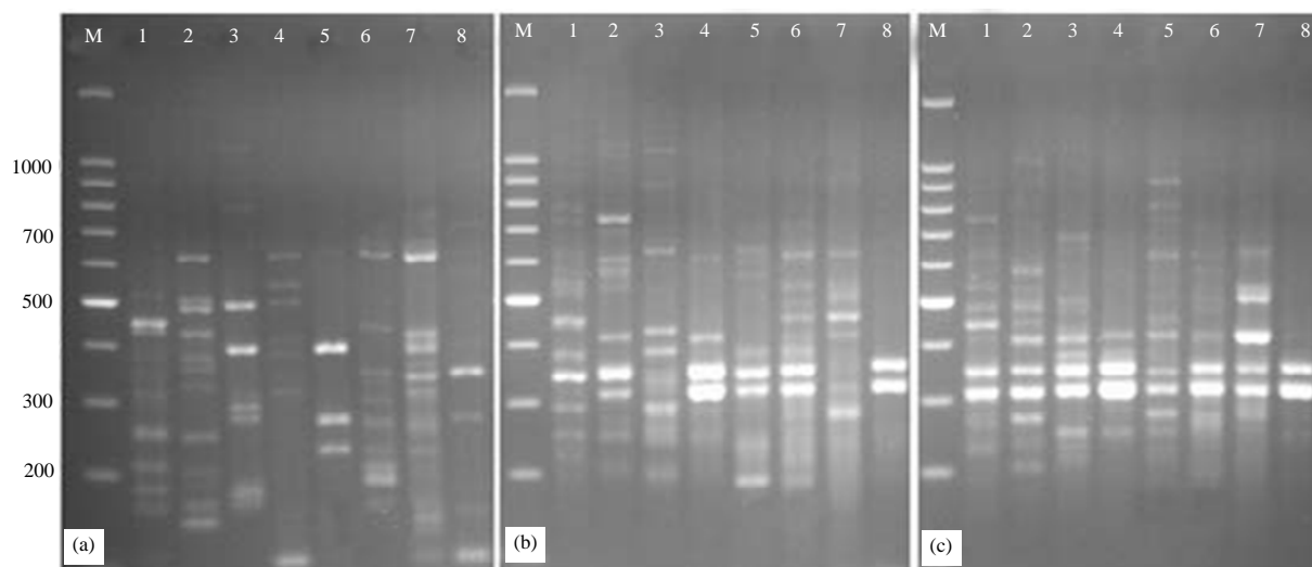
Fig. 5: Rep-PCR profiles of eight mycoplasma isolates, (a) Rep-I5, (b) Rep-I7 and (c) Rep-I8
