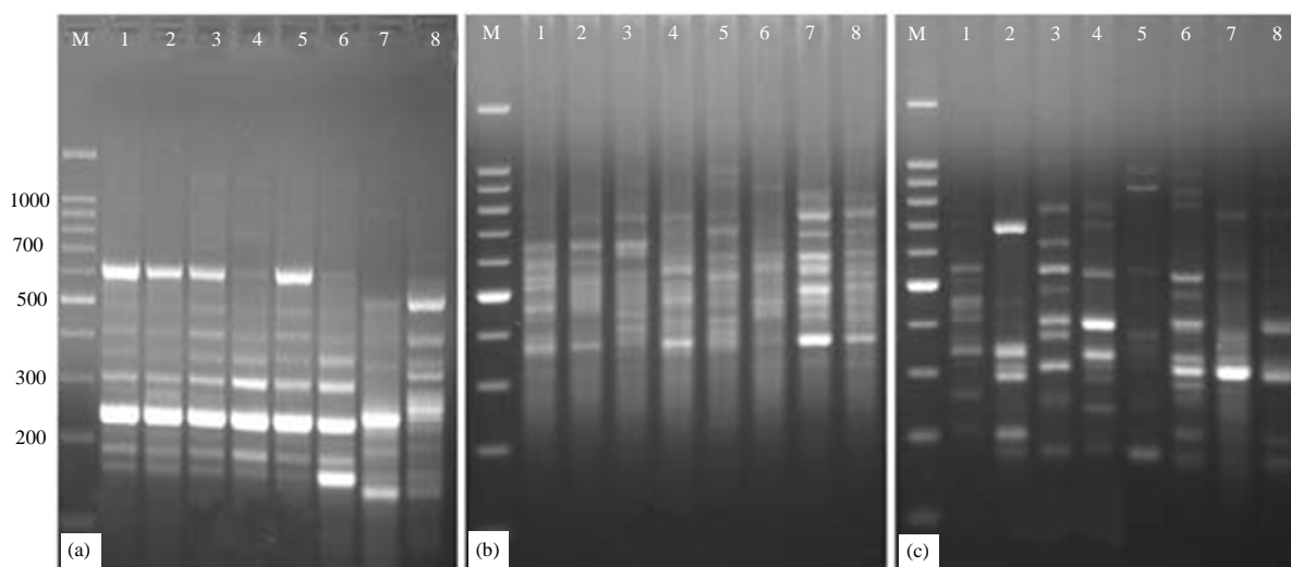
Fig. 4: Rep-PCR profiles of eight Mycoplasma isolates (a) BOX AI, (b) Rep-I10 and (c) Rep-I12 Lane1 = M: 100-bp DNA ladder and Lane 2-9: Mycoplasma strains
