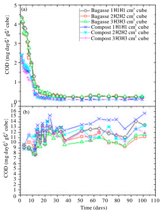
Fig. 1: (a) COD releasing rate from oxygen releasing material and (b) DO concentration from oxygen releasing material
