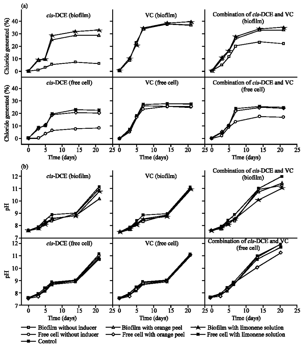
Fig. 4: (a) Percentage of chloride generated and (b) pH in microcosm study
