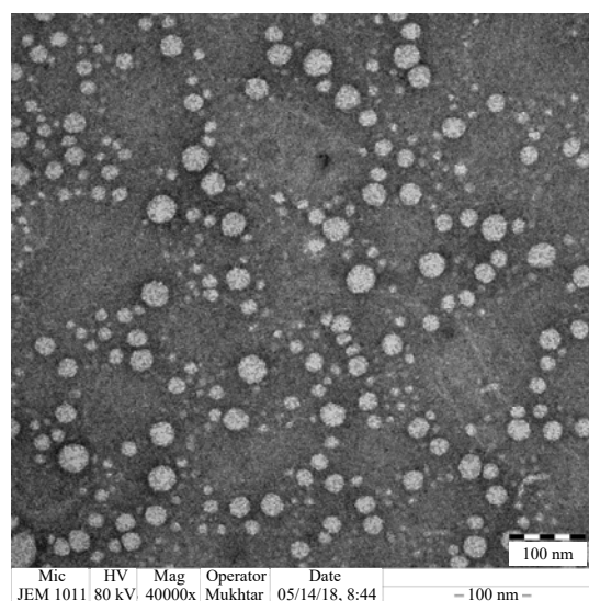
Fig. 1: Transmission electron microscopic (TEM) image of optimized LiC-ThA NSLCs formulation
