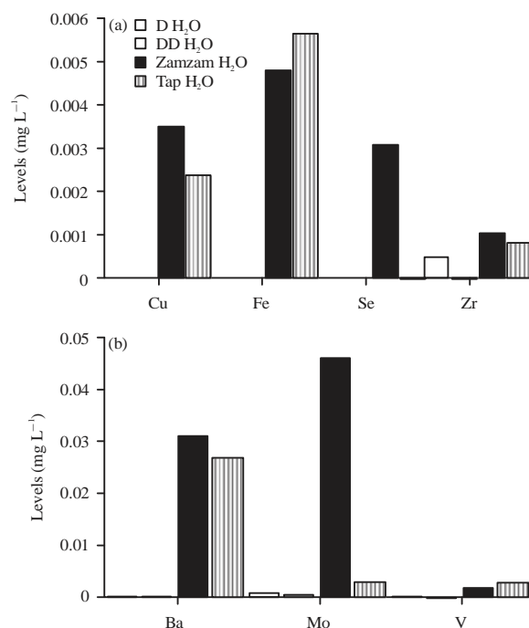
Fig. 3(a-b): The traces and some anticancer elements (Se, V and Fe) in Zamzam water compared to tap water (TW)
