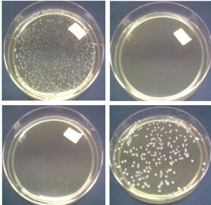
Fig. 2: The performance of isolated LABs after 48 h incubation on 42°C temperatures
