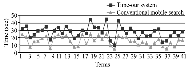
Fig. 3: Time taken for first query output
