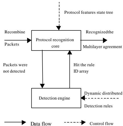
Fig. 2: UAEE engine basic architecture
