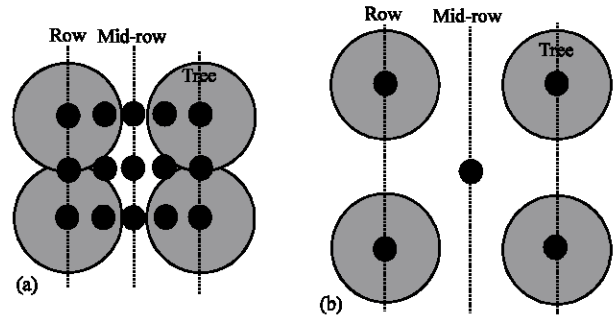
Fig. 1: Position of vegetation area index measurements (black points) with plant canopy analyzer LAI-2000 and hemispherical photograph. (a) Saada 1, with high ground cover f_c = 0.7 and (b) Saada 2, with low ground cover f_c = 0.3
