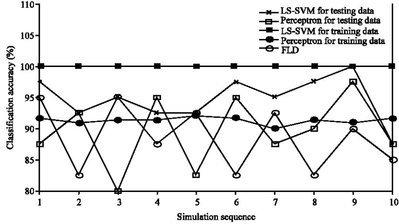
Fig. 3: Classification accuracy with LS-SVM, perceptron and FLD for 10 separate simulations
