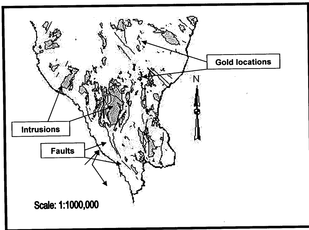
Fig. 4: Combined Layer of Gold Locations, Faults and Intrusions, Southern Arabian Shield
