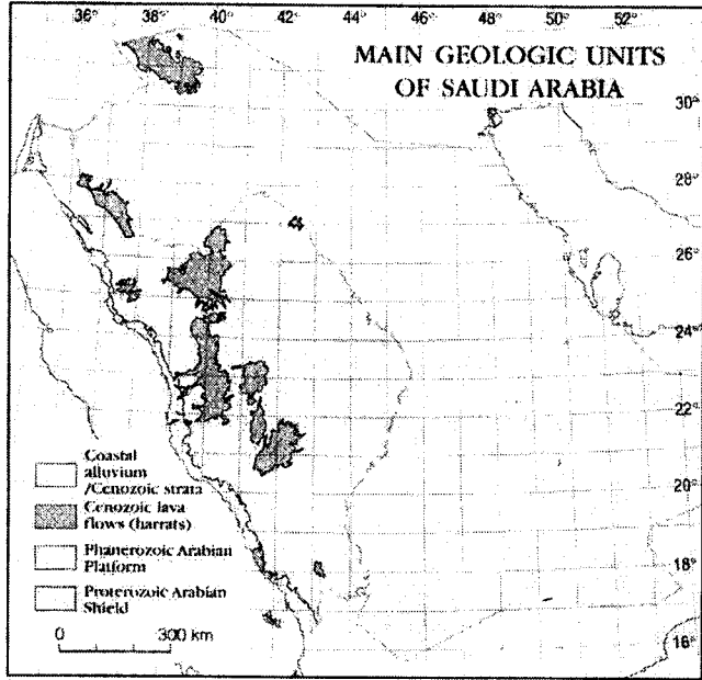
Fig. 1: The Main Geological Units of Saudi Arabia (From Collenette and Grainger, 1994)
