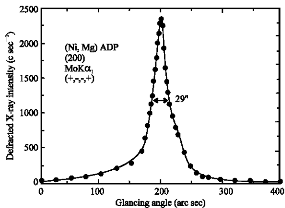
Fig. 9: HRXRD of (Ni 2+ , Mg 2+ ) ADP crystal
