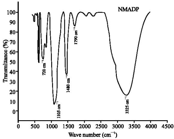
Fig. 4: FTIR spectrum of (Ni-Mg) ADP crystal
