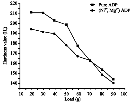
Fig. 6: Microhardness curve of pure and bimetallic ADP
