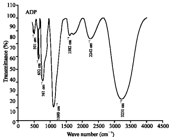
Fig. 3: FTIR spectrum of pure ADP crystal
