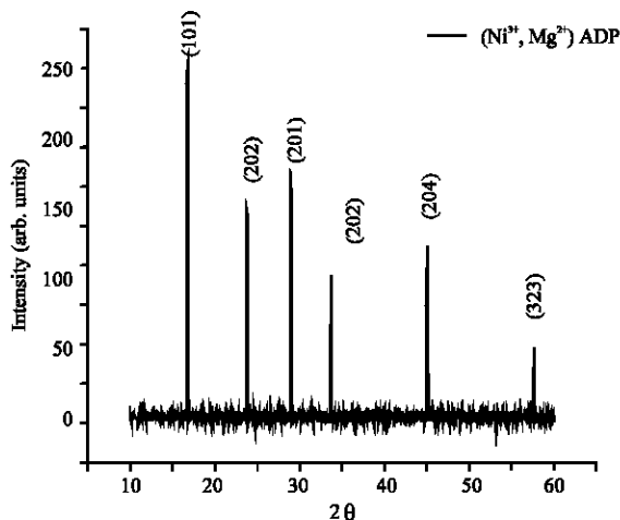
Fig. 2: Powder XRD of (Ni 3+ -Mg 2+ ) ADP
