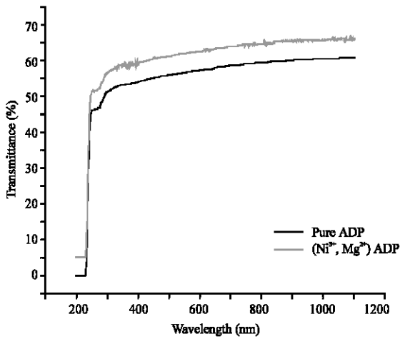
Fig. 7: UV-Vis-NIR spectra of ADP and bimetallic ADP
