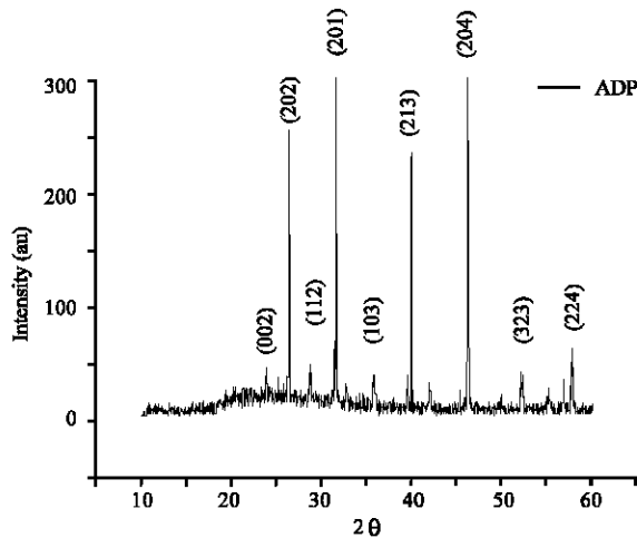
Fig. 1: Powder XRD of pure ADP crystal
