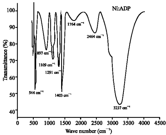
Fig. 5: FTIR spectrum of Ni: ADP crystal
