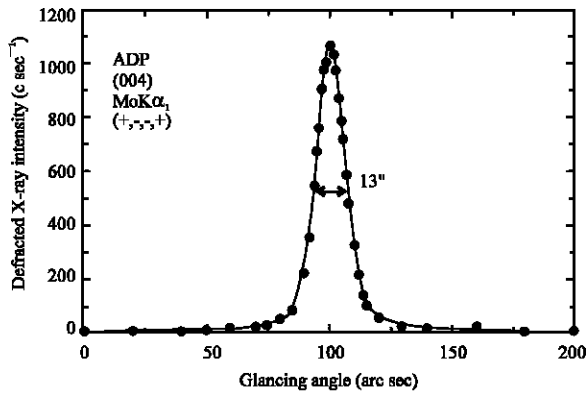
Fig. 8: HRXRD of pure ADP crystal
