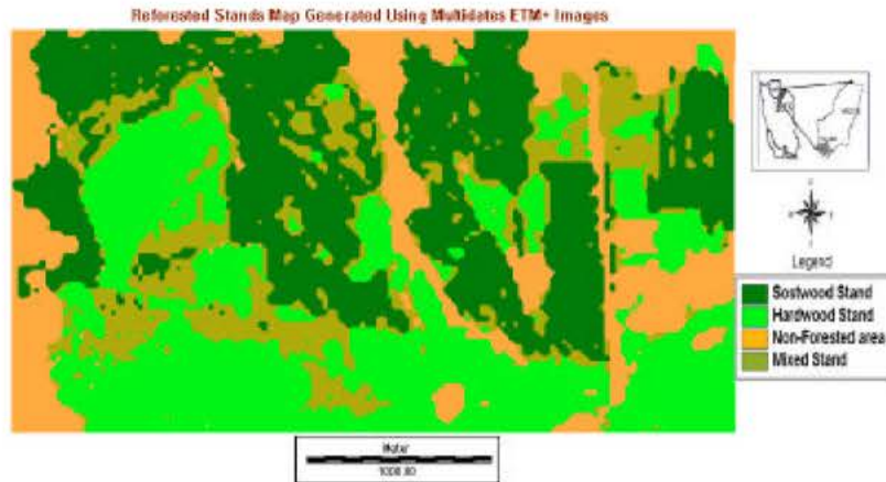
Fig. 3: The classification map of reforested types using multi-dates ETM+ images
