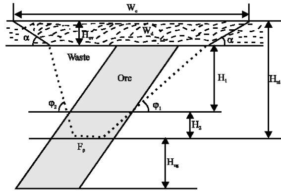
Fig. 4: TD of tabulate deposit including overburden and minimum possible width of pit floor
