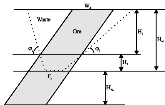
Fig. 2: TD of tabulate deposit with outcrops and including minimum possible width of pit floor
