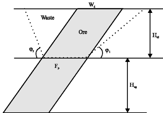
Fig. 1: TD of tabulate deposit with outcrops and including maximum width of pit floor
