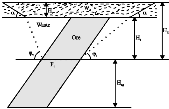
Fig. 3: TD of tabulate deposit including overburden and maximum width of pit floor
