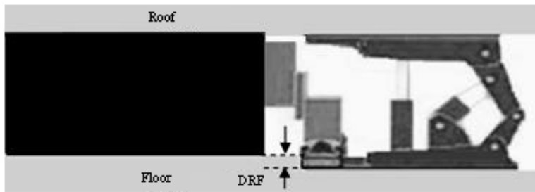
Fig 2: Depth of Removing Floor (DRF) by shearer on a soft floor in longwall
