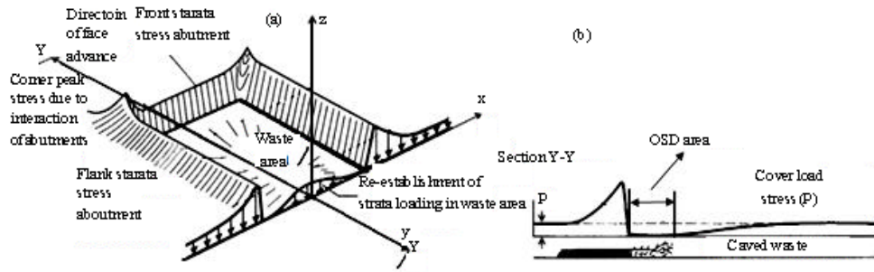
Fig. 7: Vertical stress redistribution in the plane of the seam around a longwall coal face (a) and OSD area in front of the face (b) (Richard et al. , 1998)
