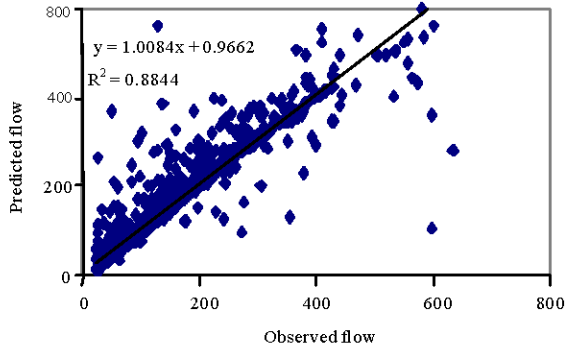
Fig. 2: Scattering graph of predicted against measured flow (cms) in K-NN model
