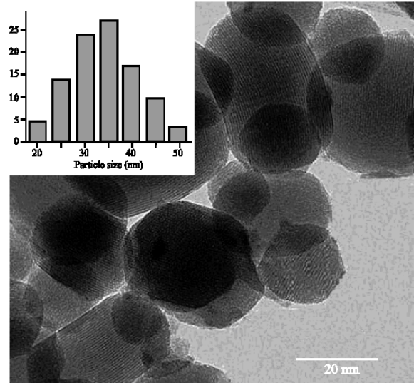
Fig. 3: TEM image of Zn 0.9 Mn 0.1 O nanopowder calcinated at 400°C. The inset presents its particle size distribution
