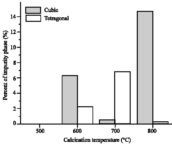
Fig. 2: Bar diagrams present an approximation on each of secondary phases' percentage in Zn 0.9 Mn 0.1 O samples calcinated at 500-800°C
