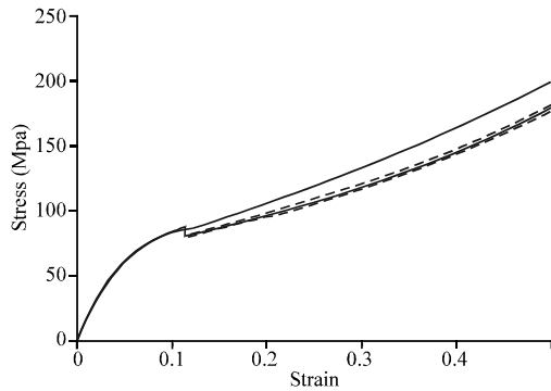
Fig. 9: Measured static and RU compression test for lubricated surface showing: — static and mean stress, ---- path of max. and min. oscillatory stress
