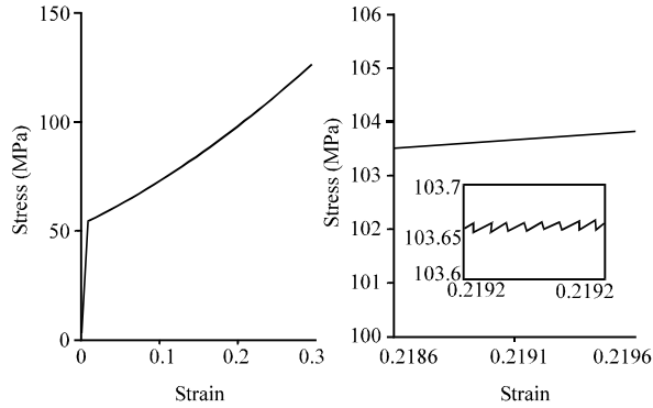
Fig. 5: FE model showing an interval of RU excitation for zero friction, \mu = 0 , inset shows zoomed in view of oscillatory stress amplitude
