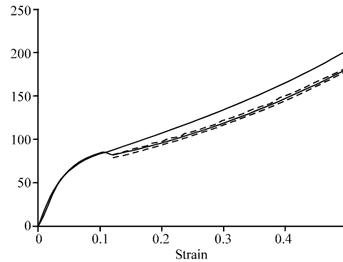
Fig. 4: Measured static and RU compression test for dry surface showing: — static and stress, ---- path of max. And min. oscillatory stress (Daud and Lucas, 2007)
