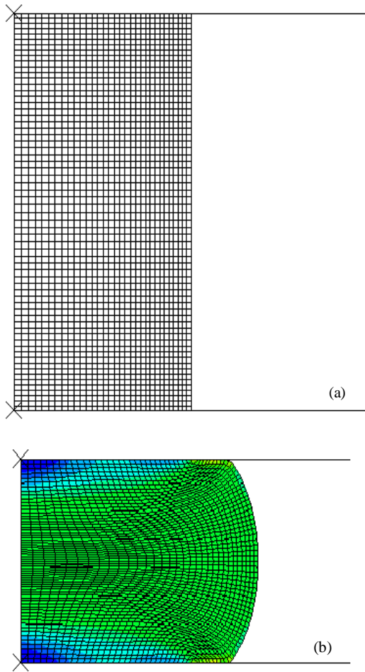
Fig. 2: (a) Original and (b) deformed mesh profiles of a cylindrical specimen model
