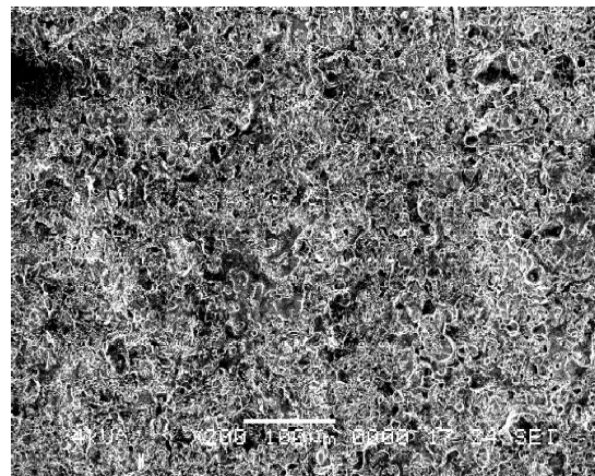
Fig. 1C: Run 5 (I = 23 A, V = 40 V: Dry-WEDM, R_a = 1.72 \mu\text{m} )
