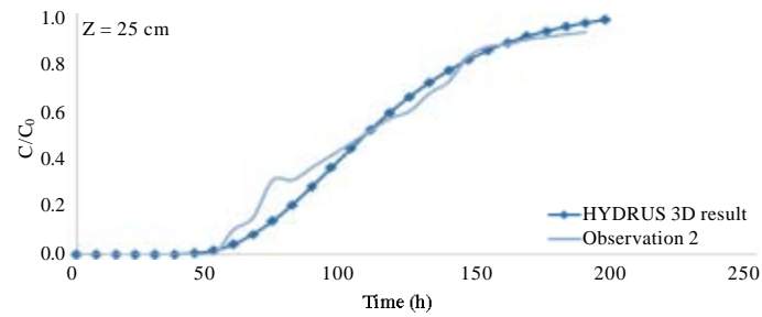
Fig. 9: BTC curve from experimental and HYDRUS-3D second test at 25 cm depth
