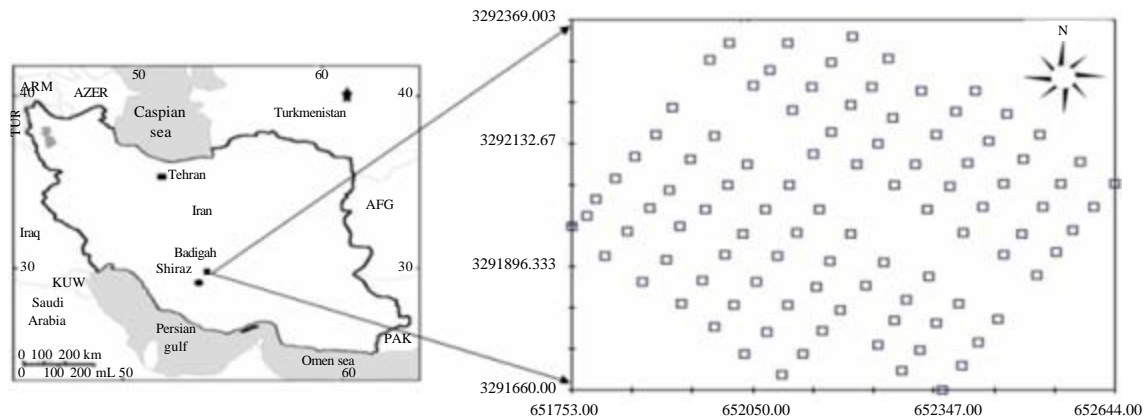
Fig. 1: Location of the study area and sampling pattern in 46.7 ha area
