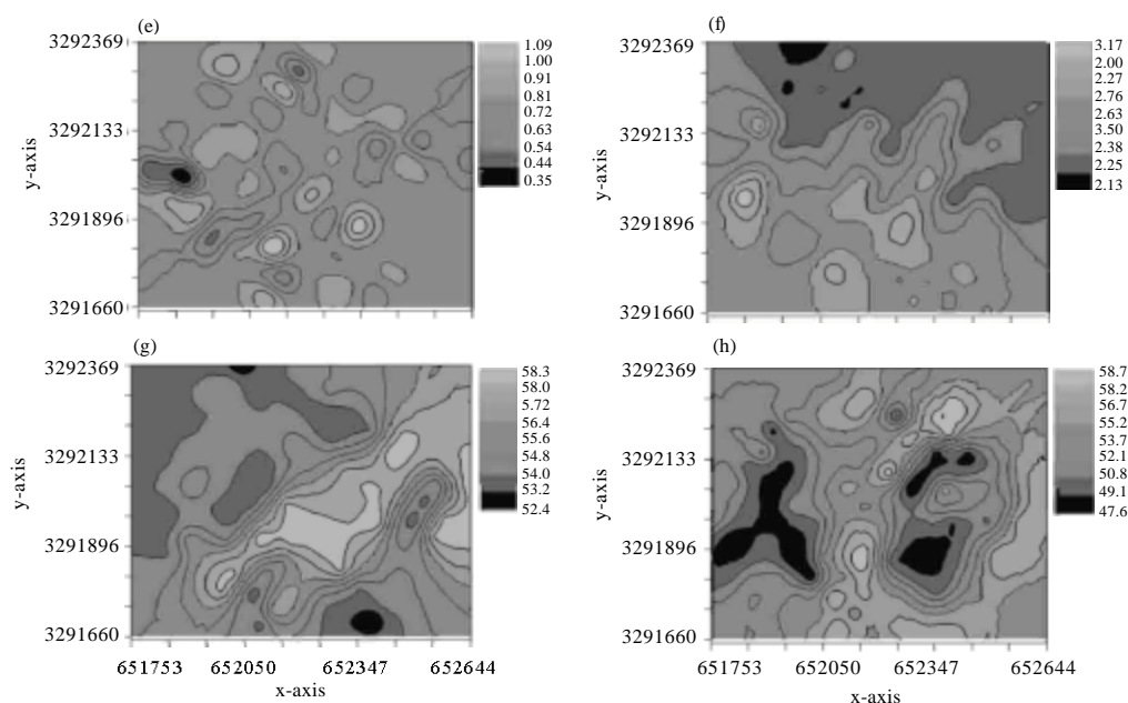
Fig. 5(a-h): Digital maps of soil properties prepared by ordinary kriging, (a) Silt (%), (b) Sand (%), (c) Mn ( \text{mg kg}^{-1} ), (d) Fe ( \text{mg kg}^{-1} ), (e) ECE ( \text{ds m}^{-1} ), (f) Ca ( \text{mg kg}^{-1} ), (g) Clay (%) and (h) CCE (%)
