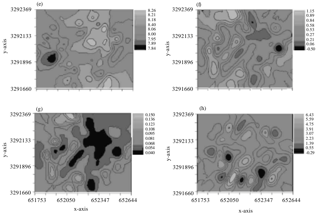
Fig. 4(a-h): Digital maps of soil properties prepared by ordinary kriging, (a) CEC (Cmol kg -1 ), (b) Ca (meq L -3 ), (c) pH, (d) P (mg kg -1 ), (e) pH, (f) OM (%), (g) TN (%) and (h) Mg (meq L -3 )
