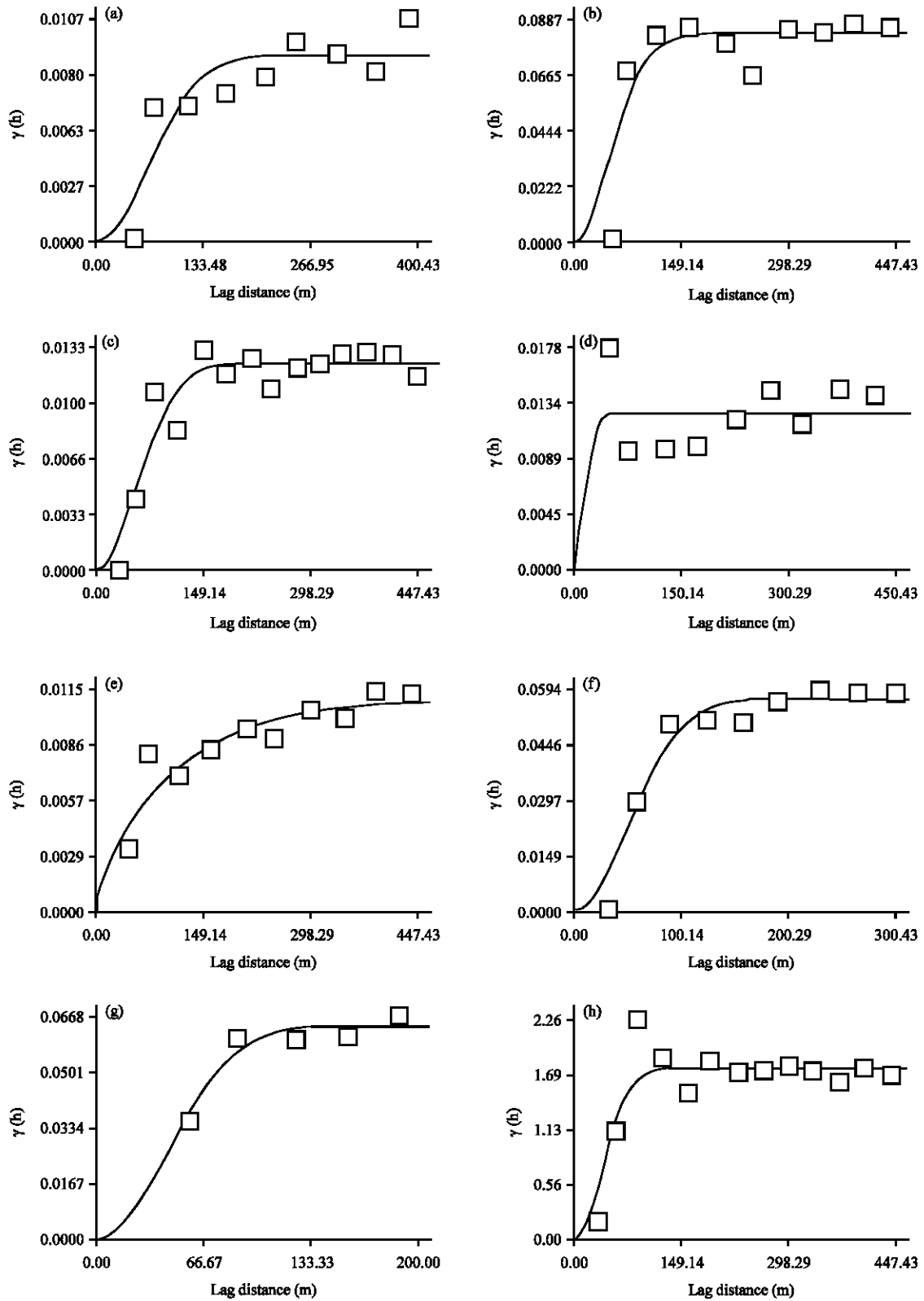
Fig. 2(a-h): Omnidirectional semivariogram for soil parameters, (a) CEC, (b) Ca, (c) K, (d) P, (e) pH, (f) OM, (g) TN and (h) Mg
