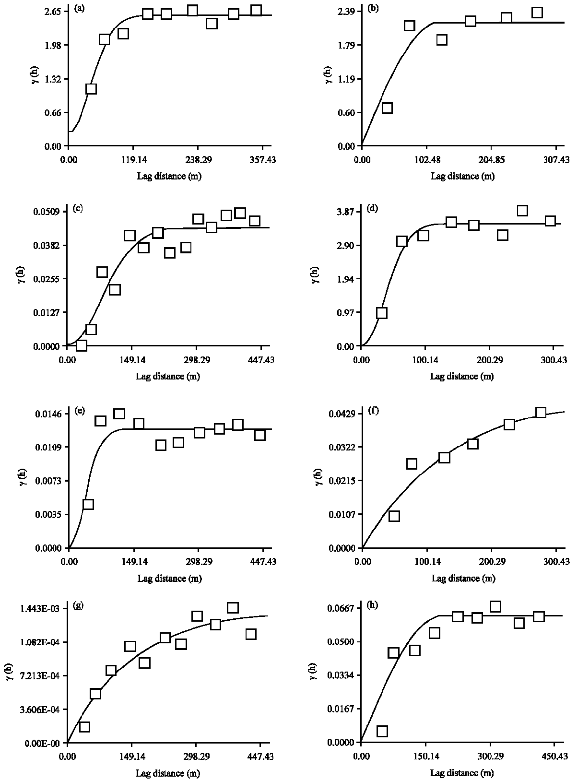
Fig. 3(a-h): Omnidirectional semivariogram for soil parameters, (a) Silt, (b) Sand (c) Mn, (d) Fe, (e) ECe, (f) CU, (g) Clay and (h) CCE
