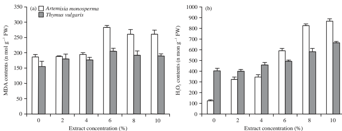
Fig. 7(a-b): Allelopathic effects of Artemisia monosperma and Thymus vulgaris leaf aqueous extract on (a) Malondialdehyde (MDA) and (b) \text{H}_2\text{O}_2 ( \text{nmol g}^{-1} \text{FW} ) of pea ( Pisum sativum L.) seedlings. Vertical bars represent \pm SD
