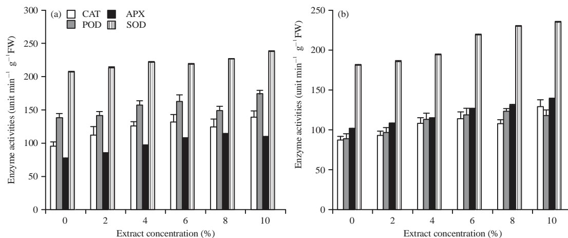
Fig. 6(a-b): Allelopathic effects of (a) Artemisia monosperma and (b) Thymus vulgaris leaf aqueous extract on enzymes activity (CAT, POD, APX and SOD) ( \text{Unit min}^{-1} \text{g}^{-1} \text{FW} ) of pea ( Pisum sativum L.) seedlings. Vertical bars represent \pm SD
