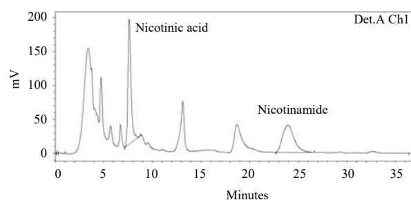
Fig. 3: HPLC chromatogram of nicotinic acid and nicotinamide in the tomato sample under chromatographic conditions of the analytical method
