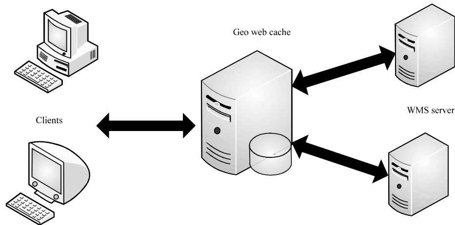
Fig. 5: GeoWebCache service framework
