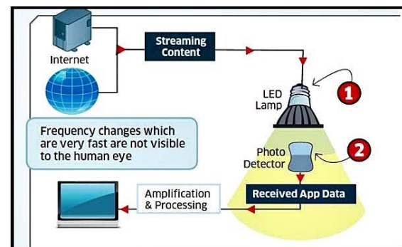
Fig. 2: Different phases for the operation of Li-Fi system Source: Dimitrov and Hass 1 and Hase et al. 5
