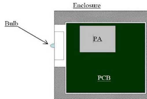
Fig. 1: Block diagram of Li-Fi sub-assemblies Source: Gupta 15 and Sharma and Sanganal 17
