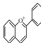
Fig. 1: Flavylium cations structure
