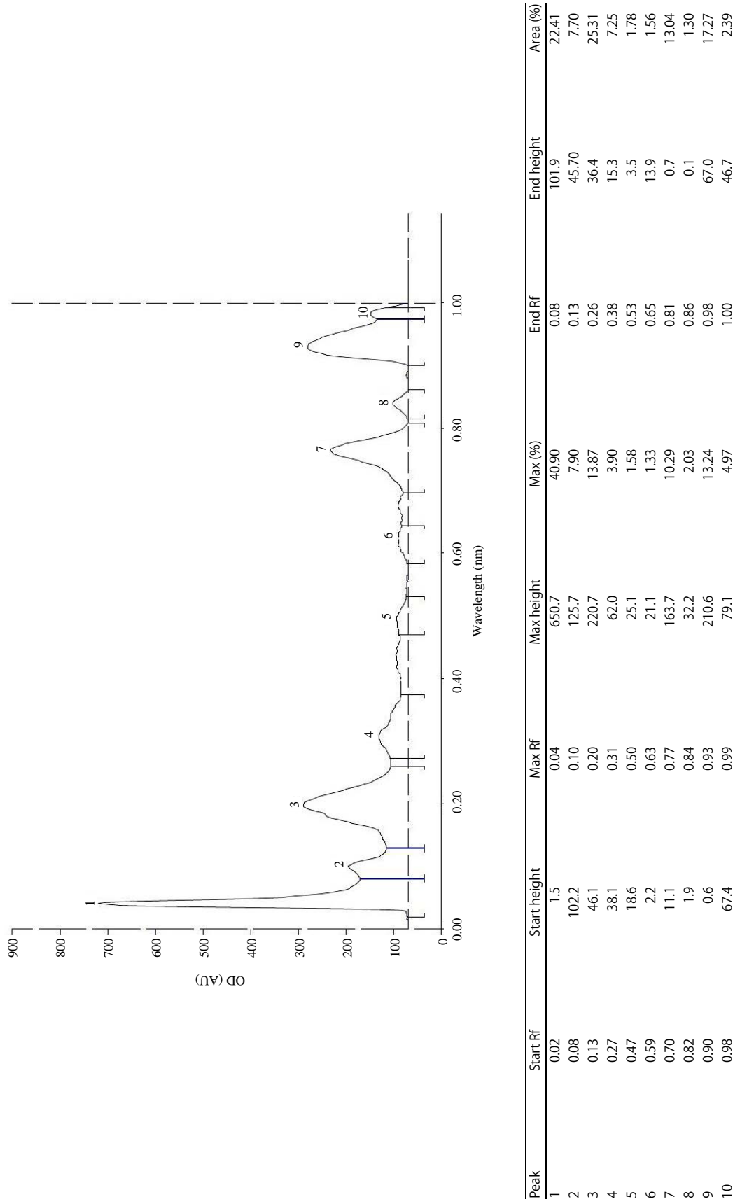
Fig. 9: HPTLC profile of in vitro raised plant after 20 days at 254 nm
