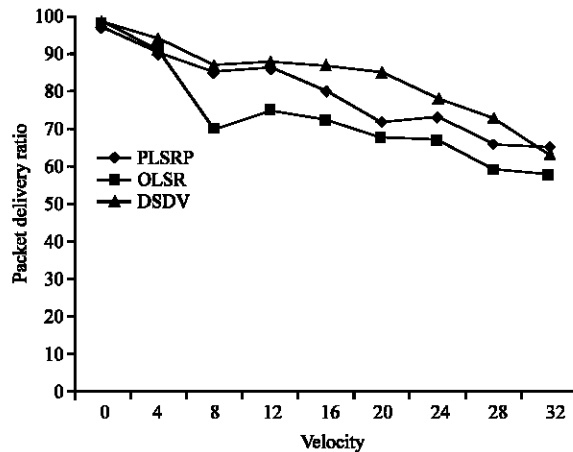
Fig. 3: Packet delivery ratio vs. node velocity
