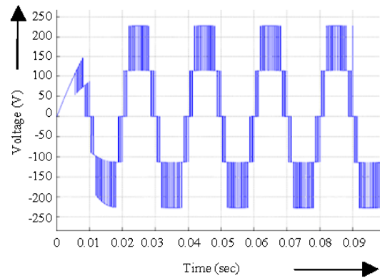
Fig. 6: Proposed inverter output voltage
