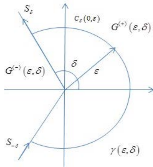
Fig. 1: Hankel contour
