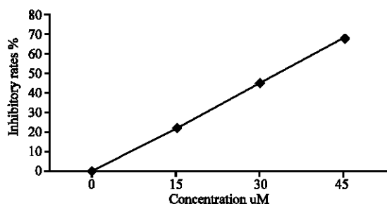
Fig. 6: Dose- response curve of \alpha -anordrin addition to CaM activated \text{Ca}^{++}\text{-Mg}^{++}\text{-ATPase} activity
