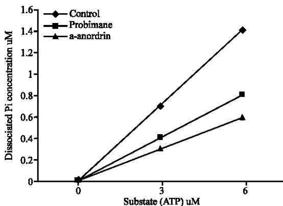
Fig. 4: Substrate (ATP)-response curve. Probimane (30 μM) and α-anordrin (10 μM) on membrane solution (CaM and Ca ++ -Mg ++ -ATPase) with different substrate (ATP) solution (1:50 v/v) for 1 h (n=3)
