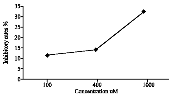
Fig. 5: Dose- response curve of low concentrations of probimane addition to CaM activated \text{Ca}^{++}\text{-Mg}^{++}\text{-ATPase} activity
