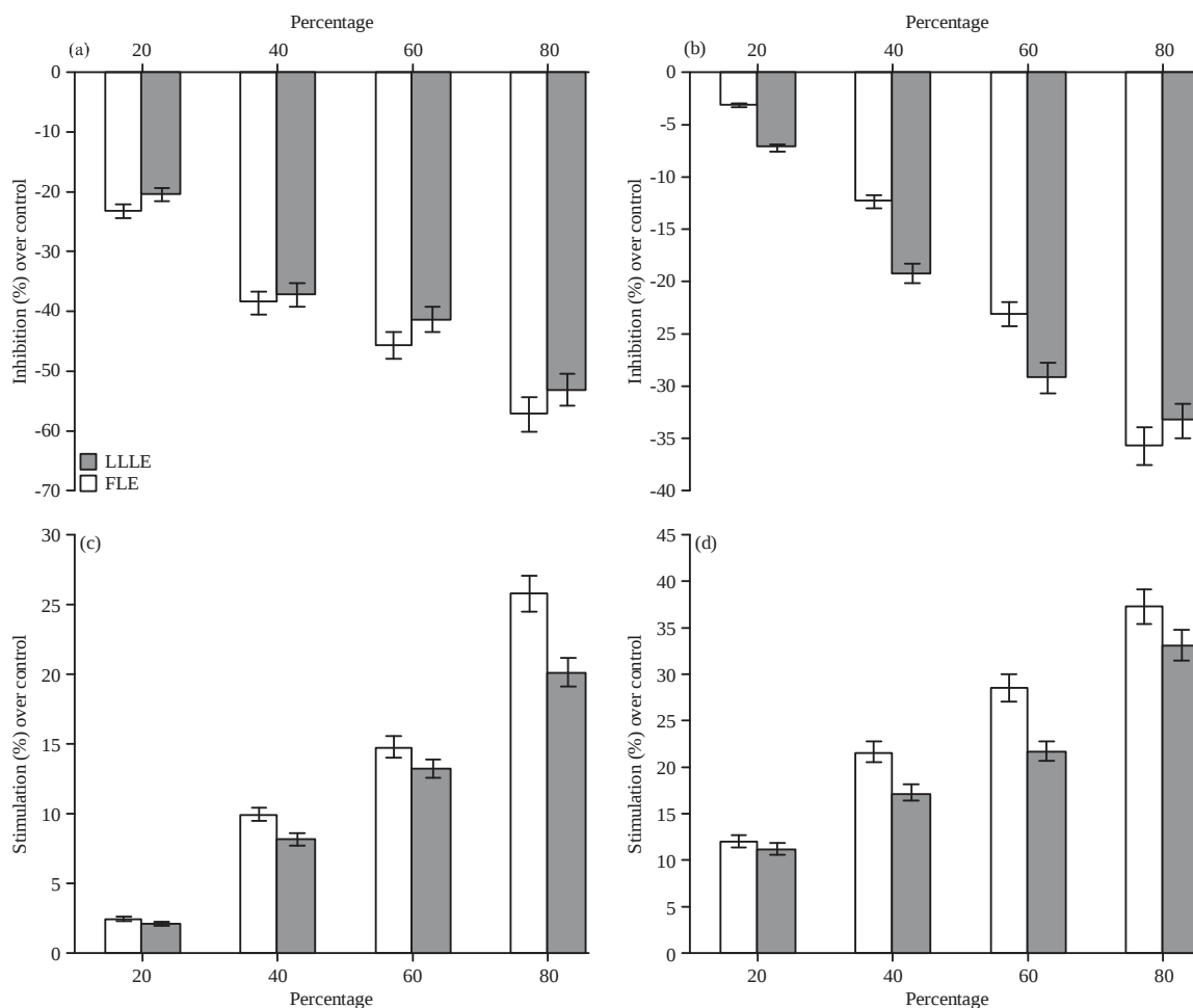
Fig. 3(a-d): Effects of fresh leaf extract (FLE) and leaf litter leachate (LLLE) extract of C. odorata on biochemical parameters of Salvadora persica , (a) Soluble protein content, (b) Total sugars, (c) Proline and (d) Phenol content
