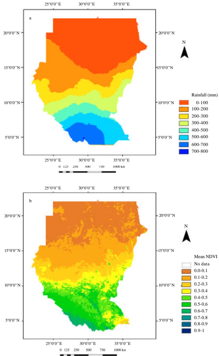
Fig. 1: (a) Average annual rainfall in Sudan (1982-1993) and (b) mean NDVI in Sudan (1982-1993)
