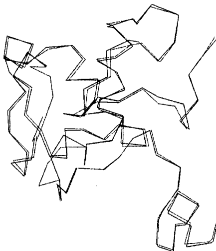
Fig. 2: Superimposition of the \alpha -carbon backbones of SoxX (Black) on the B chain of 1H33 (Red)
