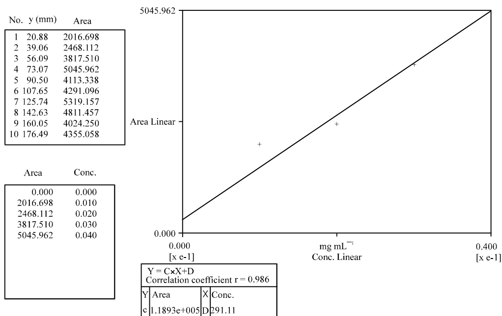
Fig. 1: The calibration curve for berberine (standard)
