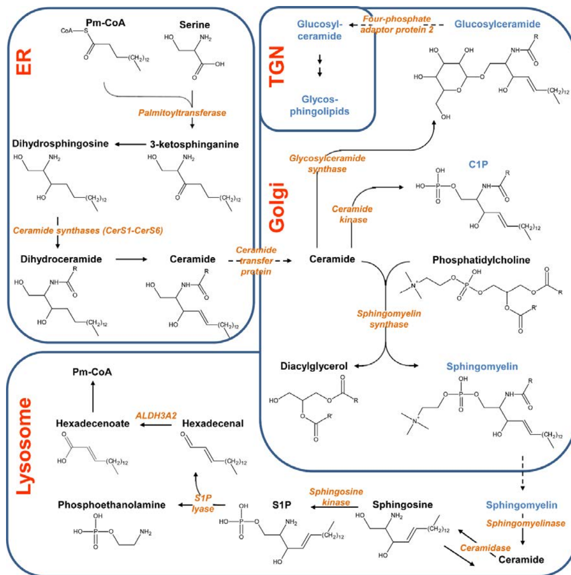
Fig. 2: Sphingolipid metabolisms. Sphingolipids are shown in blue, substrates and by-products for Sphingolipids metabolism are shown in black and all important enzymes are shown in orange. Biochemical reactions are represented by solid arrows and inter-organelle transportations are represented with dashed arrows. R and R' in represent possible functional groups derived from fatty acid. ALDH3A2: Fatty aldehyde dehydrogenase, C1P: Ceramide-1-phosphate, ER: Endothelium reticulum, Pm-CoA: Palmitoyl coenzyme A, S1P: Sphingosine-1-phosphate and TGN: Trans-Golgi network
