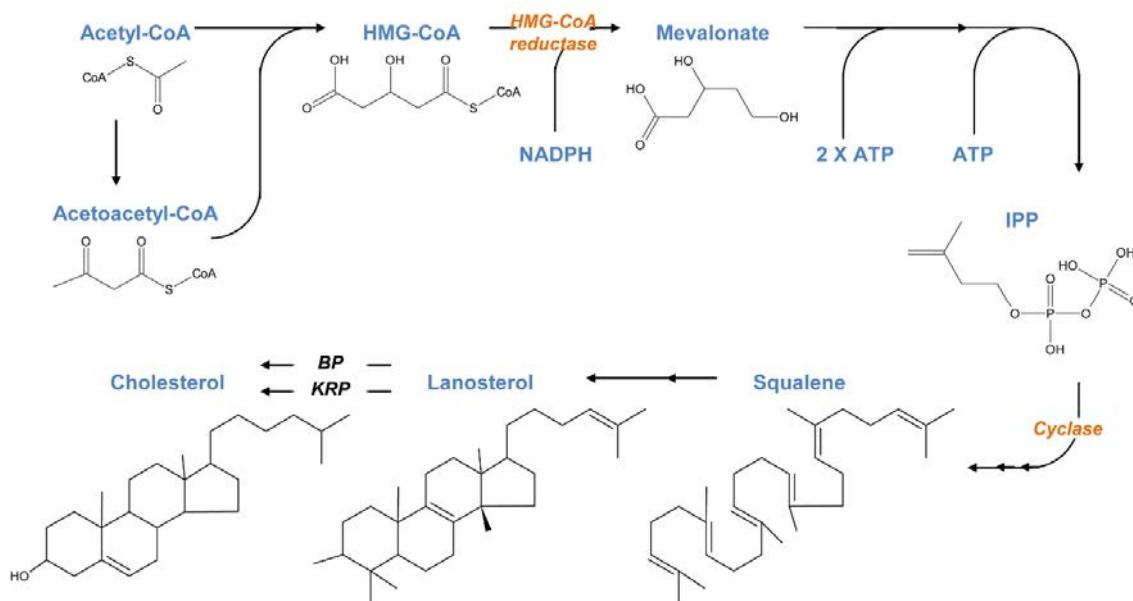
Fig. 3: Biochemical pathway of cholesterol synthesis. BP: Bloch pathway, HMG-CoA: 3-hydroxy-3-methylglutaryl-CoA, KRP: Kandutsch-russell pathway and IPP: Isopentenyl pyrophosphate
