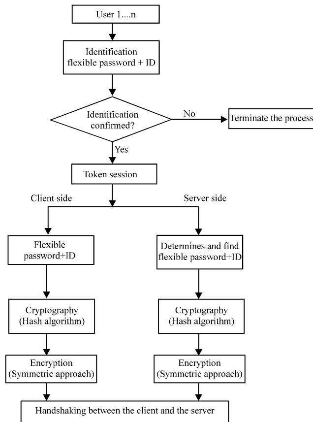
Fig. 4: Scenario of a dependable security model
